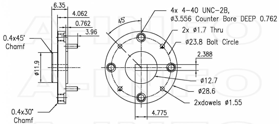
FUGP500 (equivalent to UG-383/U-M)
